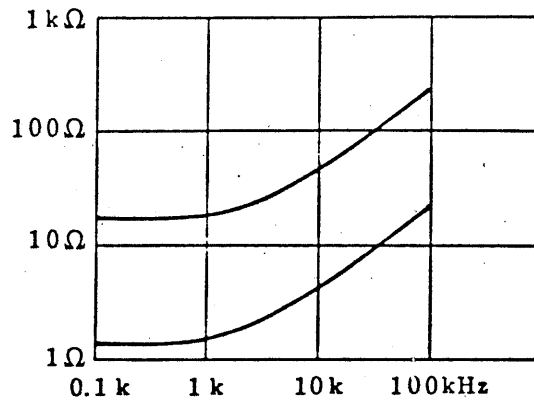
Figure 2-4-5 Impedance Characteristics of a Common Sliding Resistor
