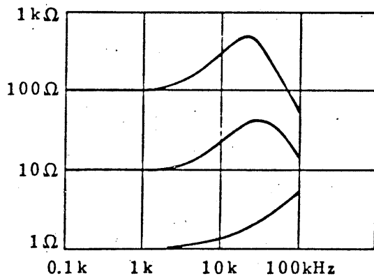
Figure 2-4-4 Impedance Characteristics of PLZ-700W
